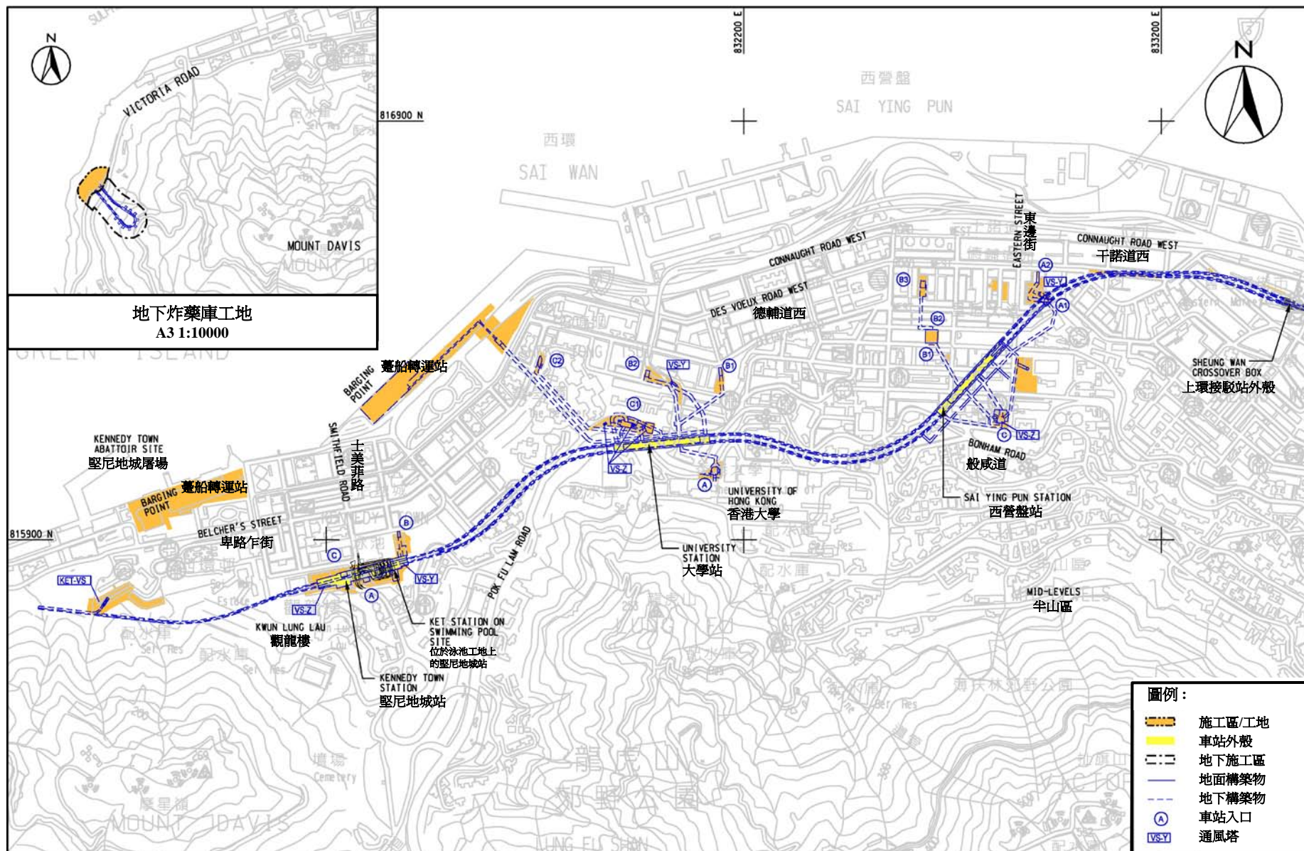
Figure 1: West Island Line Overall View 圖 1: 西港島綫全綫示意圖
